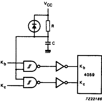
Fig.14 External circuit for master preset at start-up.
